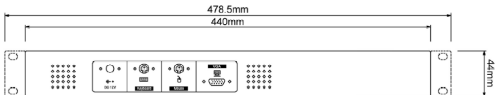
Rear out-side view (ST-17LKM1U-1C)
