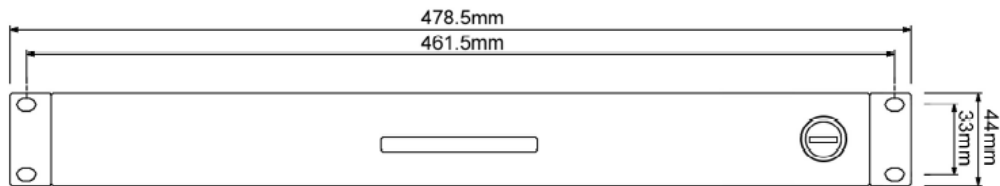
Front out-side view
